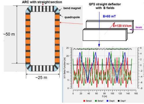
Figure 2: Second option of ring lattice based on QFS concept with TWISS.
